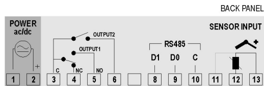
Fig. 1 – N322 terminals
