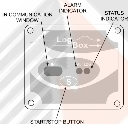
Figure 01 – Logger Front
